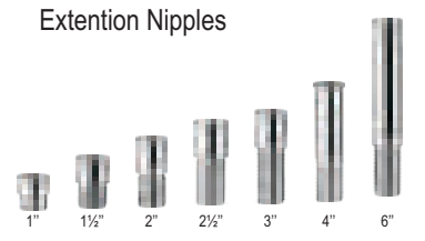
Extention Nipples
